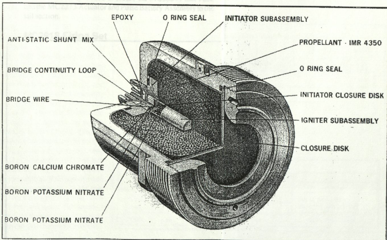
Figure 5. MC1835 Gas Generator
